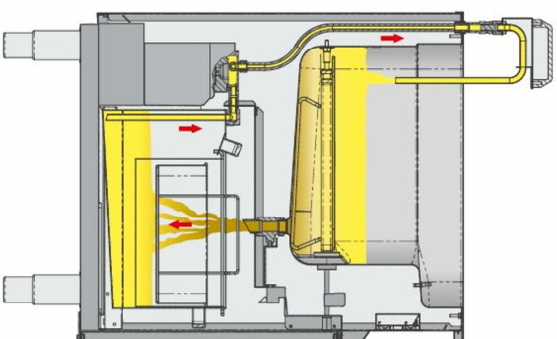
Filter pumping system
